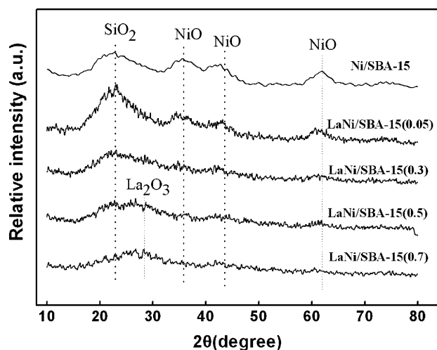
Fig. 5. Wide-angle XRD patterns of Ni/SBA-15 catalysts promoted with lanthanum oxides after calcination at 823 K for 4 h.
