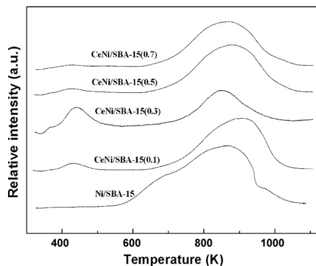
Fig. 7. TPR profiles of Ni/SBA-15 catalysts promoted with different loading of cerium.
